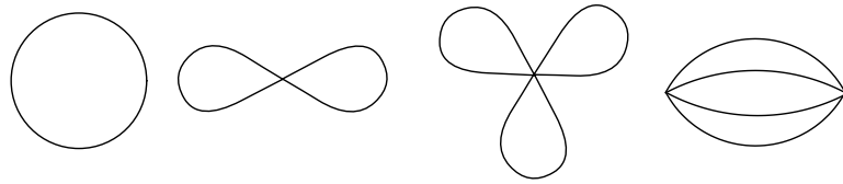
Figure 1: \mathbb{I}_0 consists of one graph (the circle). The other three constitute the set \mathbb{I}_1 . From left to right, respectively graphs 1, 2, 3, and 8 of the table.
